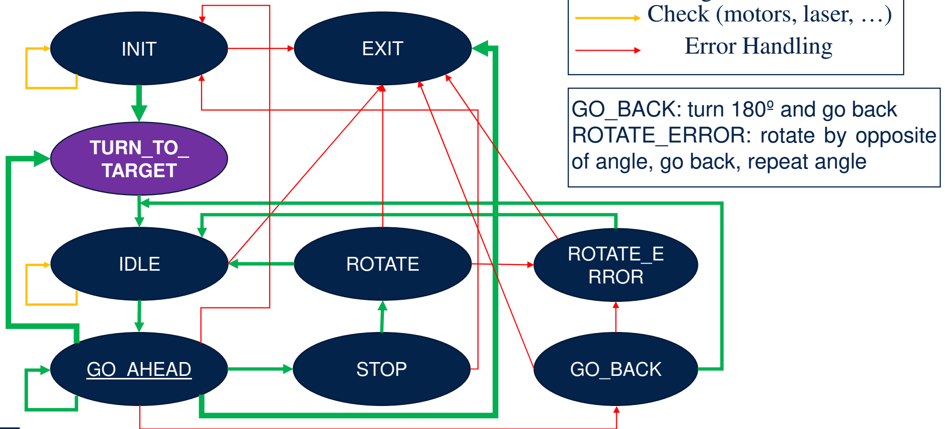
State Machine for Point to Point Navigation
